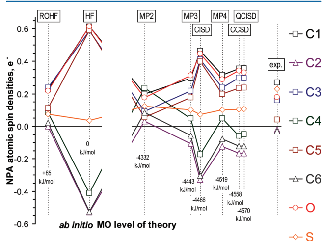
Figure 4. Ab initio wave function theory dependence of the atomic spin densities from NPA for the [Y-C] radical cofactor.
