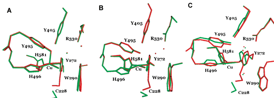
Figure 8. Overlay of optimized structures of holo-GO models in the presence (red) and absence (green) of the Tyr-Cys cross-link: (A) oxidized [Cu(II)-Y·], (B) semireduced [Cu(II)-Y], and (C) reduced [Cu(I)-Y].
