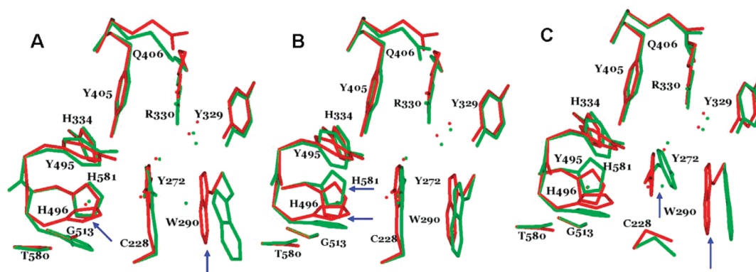
Figure 6. Overlay of initial (red) and optimized (green) geometric structures of apo-GO models: (A) apo-Y-C, (B) Y495 protonated apoH + -Y-C, and (C) Y495 protonated apoH + -Y-C without Tyr-Cys cross-link. Large structural differences are shown with a blue arrow.
